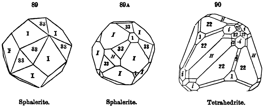
Sphalerite.
